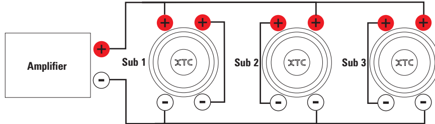
Three Subwoofer System (3) Dual 4 ohm single voice coil subwoofers = 2 ohm load
