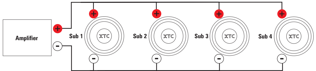
Four Subwoofer System (4) Single 4 ohm single voice coil subwoofers = 1 ohm load
