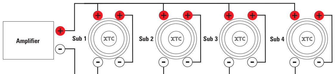
Four Subwoofer System (4) Dual 4 ohm single voice coil subwoofers = 2 ohm load
